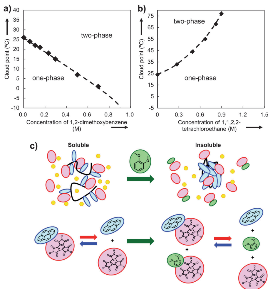
Figure 4. a,b) Cloud point ( \blacklozenge = LCST) of PPMA in 1,2-dichloroethane in the presence of 5 versus the concentration of 1,2-dimethoxybenzene (a) or 1,1,2,2-tetrachloroethane (b). [PPMA] = 10 \text{ g L}^{-1} ( 0.035 \text{ M} with respect to the pyrene units in the polymer), [ 5 ] = 0.025 \text{ M} , scan rate = 1^\circ \text{C min}^{-1} . The dashed lines show the assumed boundaries between types of thermoresponsivity. c) Presumed mechanism of the competitive effect.
