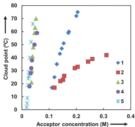
Figure 3. Dependence of the cloud point of PPMA in 1,2-dichloroethane on the concentration of the effector for effectors 1–5. [PPMA] = 10 g L -1 (0.035 M with respect to the pyrene units in the polymer).
