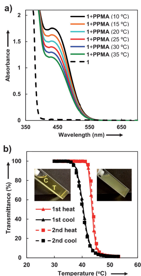
Figure 2. a) UV/Vis spectra of 1 in 1,2-dichloroethane with PPMA at various temperatures (solid lines) and without PPMA (dashed line). b) Transmittance (measured at 800 \text{ nm} ) as a function of temperature for PPMA with 1 in 1,2-dichloroethane (scan rate: 1 \text{ °C min}^{-1} ). For (a) and (b), [\mathbf{1}] = 0.14 \text{ M} , [\text{PPMA}] = 10 \text{ g L}^{-1} ( 0.035 \text{ M} with respect to the pyrene units in the polymer).
